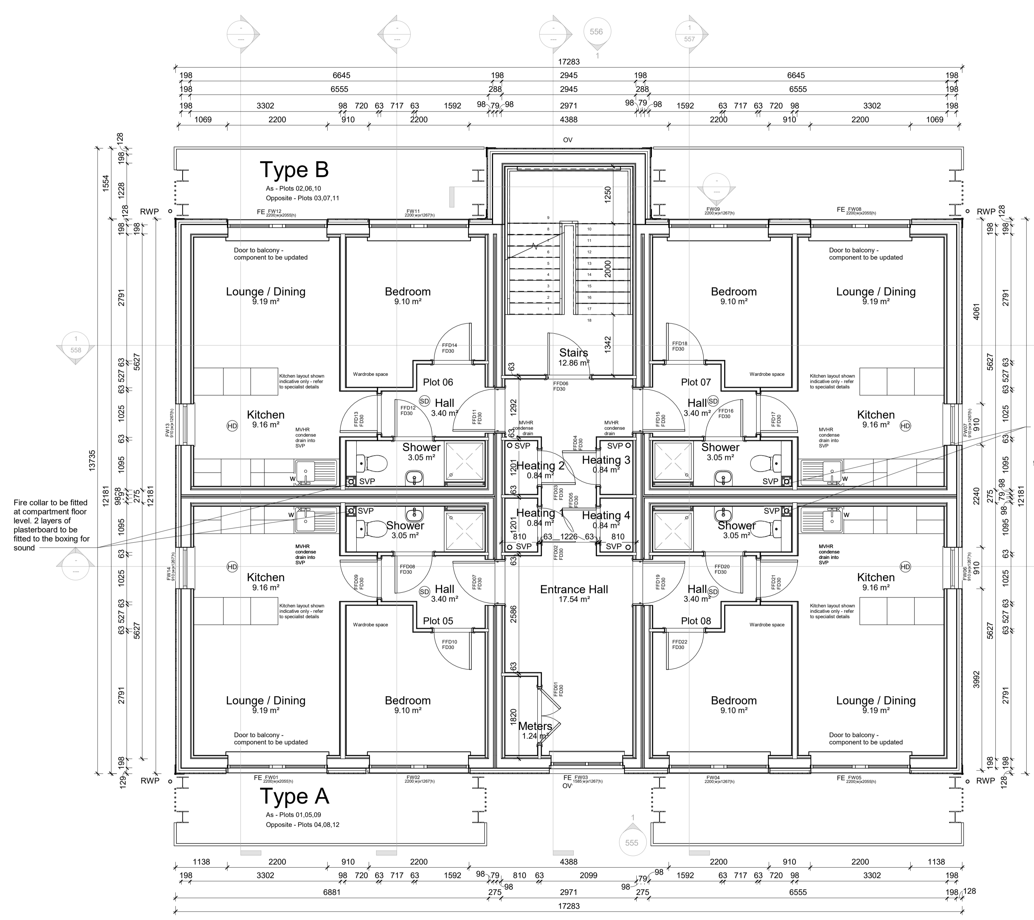
03 First floor Plan 1 : 50
