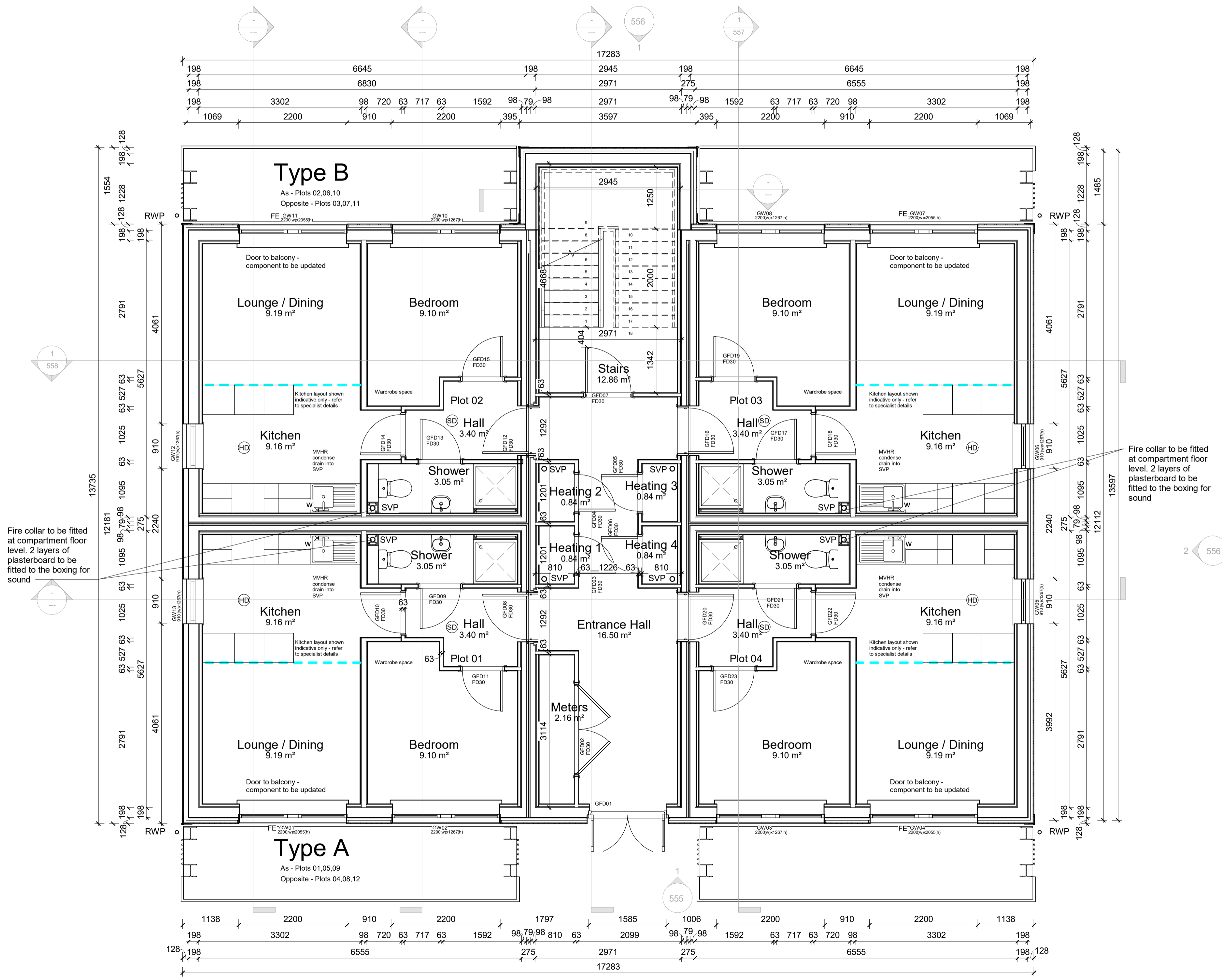
02 Ground floor Plan 1 : 50
